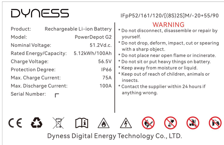
Figure 1-1 Battery Energy Storage System nameplate
