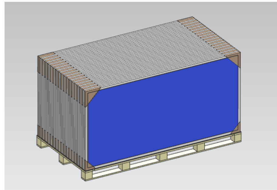
Step 4 Place subsequent modules one by one in the same side & direction on the pallet vertically
