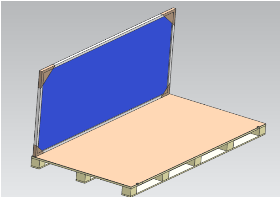
Step 3 Place the first module on the pallet vertically
